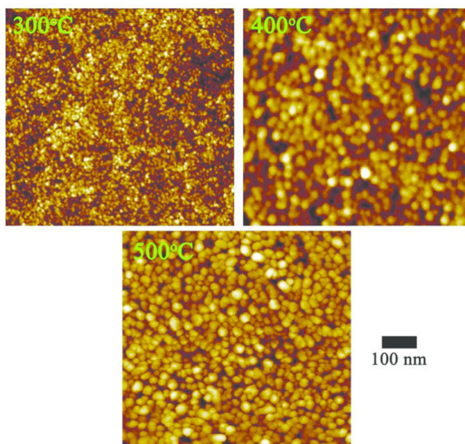
Figure 4. Atomic force microscopy (AFM) \text{TiO}_2 (Gunawan et al., 2011).
