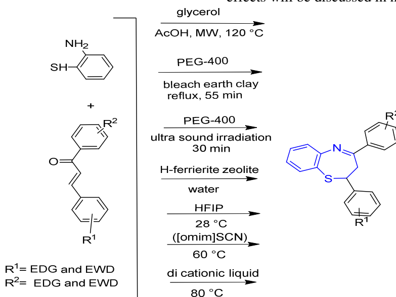
Fig. 2. Green synthetic routes to 1,5-benzothiazepines
