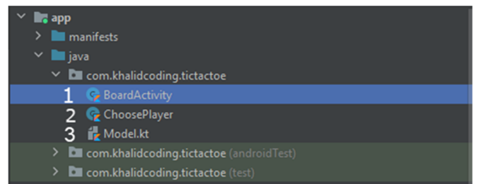
Fig. 6. Java Programming
