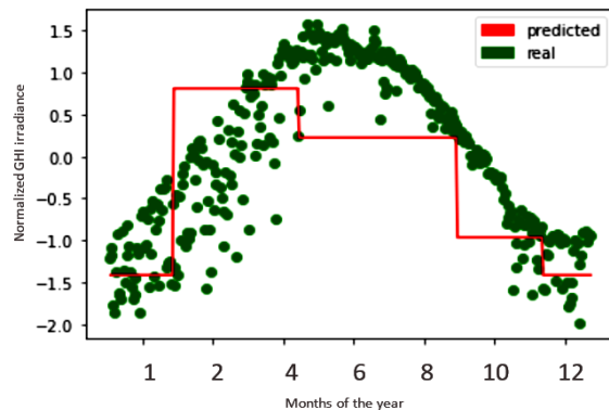
Fig. 5. Four regressors output.
