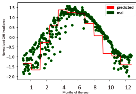
Fig. 7. Twelve regressors output.
