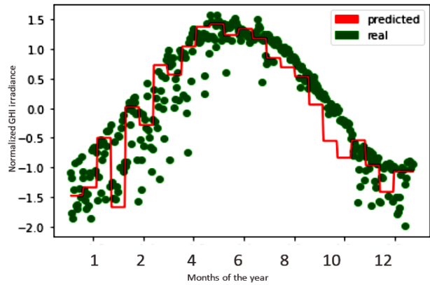
Fig. 9. Twenty-four-part regressors output
