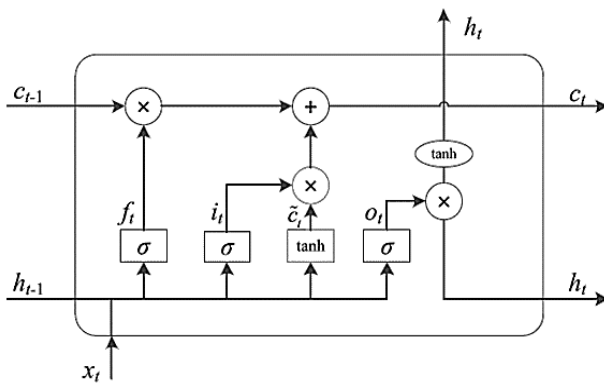
Fig. 2. LSTM structure network.
