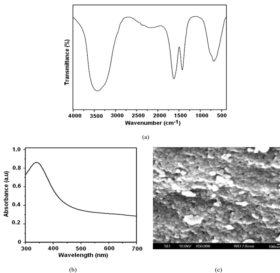
Fig. 1. Analysis results of \text{ZrO}_2 NPs: (a) FTIR spectroscopy, (b) absorption spectra, and (c) TEM image.
