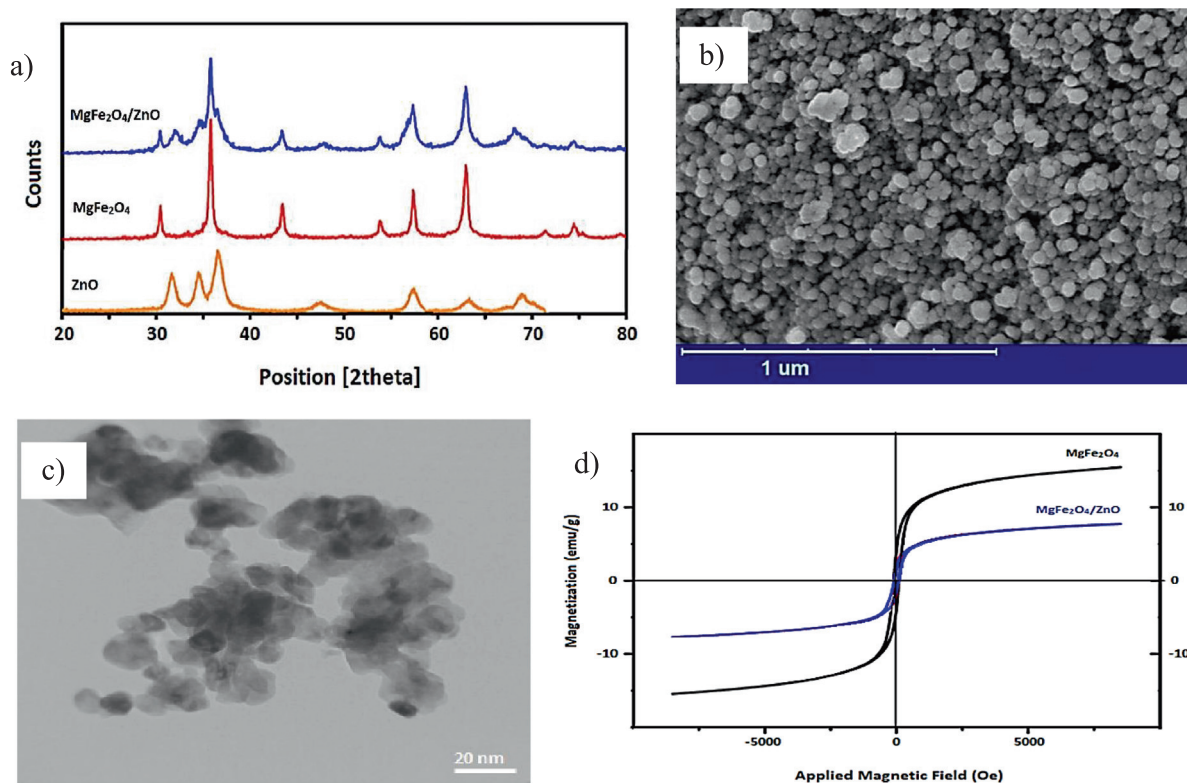
Fig. 1 A) xrd patterns, b) fesem image, c) tem image, and d) vsm spectra of mgfe 2 O 4 /ZnO nanocomposite.
